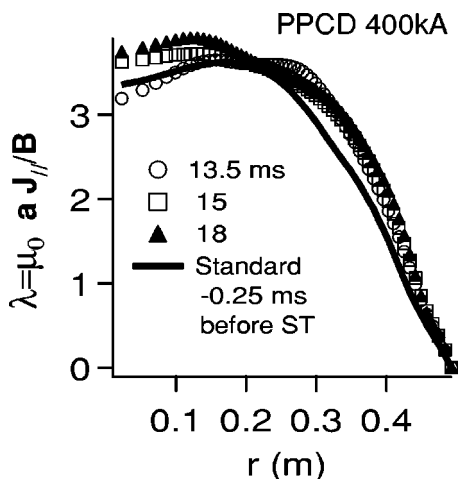
FIG. 9. A comparison of the \lambda profiles between standard and PPCD plasmas. \lambda first increases in the edge in PPCD ( \sim 13.5 ms) and then on-axis ( \sim 15 – 18 ms).
