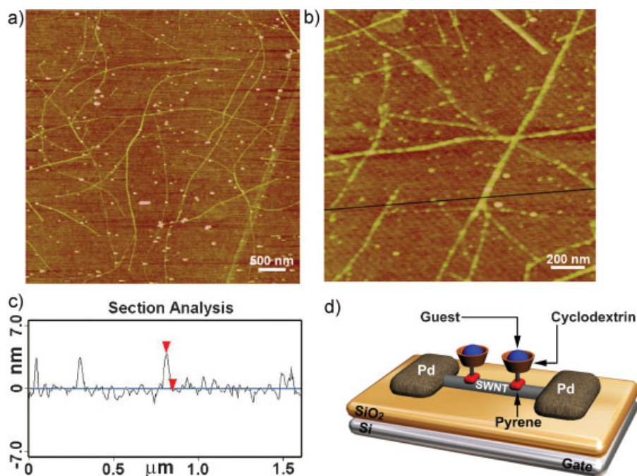
Figure 3. a) AFM image of chemical vapor deposition (CVD)-grown SWNTs with a diameter of 1.5 nm. b) AFM image of the pyrenecyclodextrin-decorated SWNTs. c) Cross-sectional analysis of (b). The height of the pyrenecyclodextrin-decorated SWNTs is estimated to be about 4.0 nm, indicating an average height for the pyrenecyclodextrin coating of around 2.5 nm. d) Model of the pyrenecyclodextrin-decorated SWNT/FET device showing how the pyrenecyclodextrin molecules interact with the SWNT and, at the same time, bind with guest molecules.
