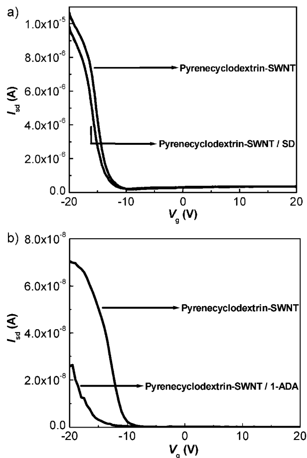
Figure 5. a) The transfer curves of the pyrenecyclodextrin-SWNT/FET devices before and after binding of the SD guest dissolved in aqueous solution at a concentration of 3.93 \times 10^{-3} \text{ mol L}^{-1} and b) the transfer curves of the pyrenecyclodextrin-SWNT/FET before and after binding of the 1-ADA guest dissolved in aqueous solution at a concentration of 3.98 \times 10^{-3} \text{ mol L}^{-1} . Both experiments were carried out at room temperature.
