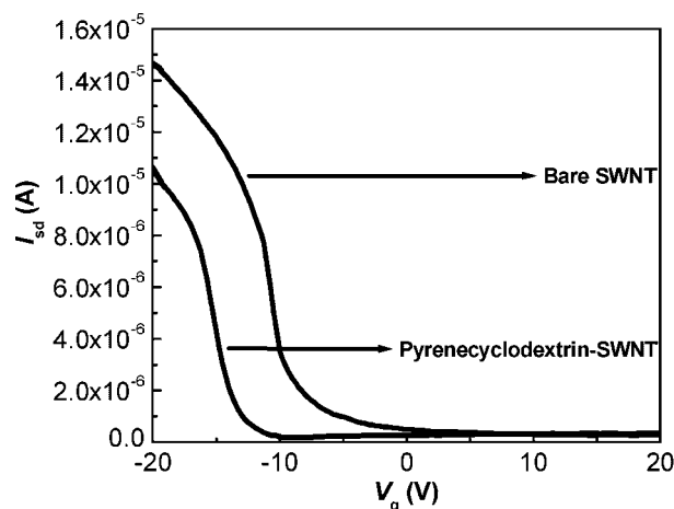
Figure 4. Transfer curves obtained from the SWNT/FET device before and after coating with pyrenecyclodextrin molecules dissolved in a DMF solution at a concentration of 1.13 \times 10^{-3} \text{ mol L}^{-1} .
