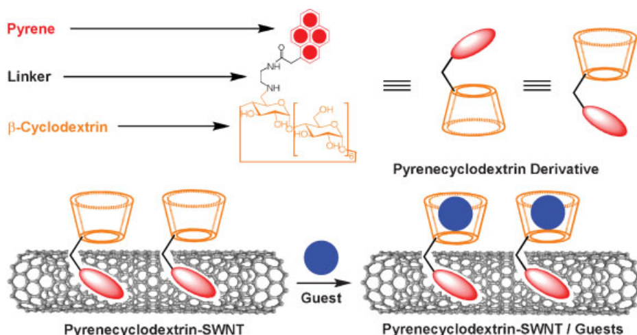
Figure 1. Schematic drawing of the pyrenecyclodextrin-decorated SWNT hybrids and how they interact with guest molecules when they are being sensed in an FET device.
