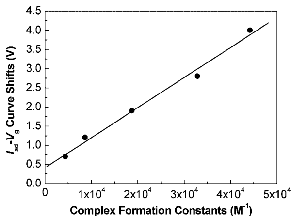
Figure 6. Plot of the curve shift values for the transfer characteristics of the pyrenecyclodextrin-SWNT/FET device, after binding different organic molecules in aqueous solution, against the K_S values for the pyrenecyclodextrin with these same organic molecules in aqueous buffer (pH = 7.0) solution.
