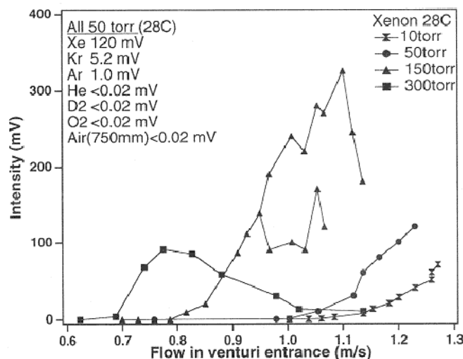
FIG. 3. Intensity as a function of flow rate for venturi cavitation with xenon in water at 28°C and various levels of saturation. At low concentration we cannot rule out the possibility that the intensity continues to increase with flow rate. Although the 150 Torr system is the brightest, it was undesirable because on the scale of seconds it would alternate between two states of different intensities at a fixed flow. Shown as a table are the maximum intensity for various gases at 50 Torr and maximum flow. For helium, deuterium, oxygen, and undegassed water any possible signal was not detectable over our noise floor (0.02 mV).
