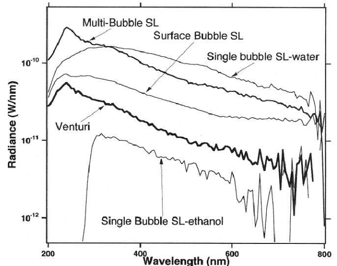
FIG. 1. Spectrum of light emitted from xenon bubbles in a venturi tube at 28 °C and 50 Torr partial pressure. Also shown for comparison are xenon spectra from surface bubble SL [14] (300 Torr, 12 °C), single bubble SL in ethanol [13] (325 Torr, -12 °C), single bubble SL in water [26] (3 Torr, 20 °C), and multibubble SL from saturated water (760 Torr, 16 °C) generated by the dipole sound field of the Contour Genesis ultrasonic-assisted liposuction device (Mentor Corporation) [14]. All data are acquired with the same equipment (10 nm FWHM resolution) and are corrected for grating and detector responses. The venturi and multibubble data are multiplied by an arbitrary factor for presentation on the graph.
