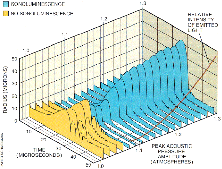
TRANSITION TO SONOLUMINESCENCE happens when the sound level reaches a critical state. The average radius of a bubble generally increases with a rise in acoustic amplitude. At the level at which sonoluminescence begins, however, the radius suddenly shrinks. The mechanism behind this transition is not understood.
